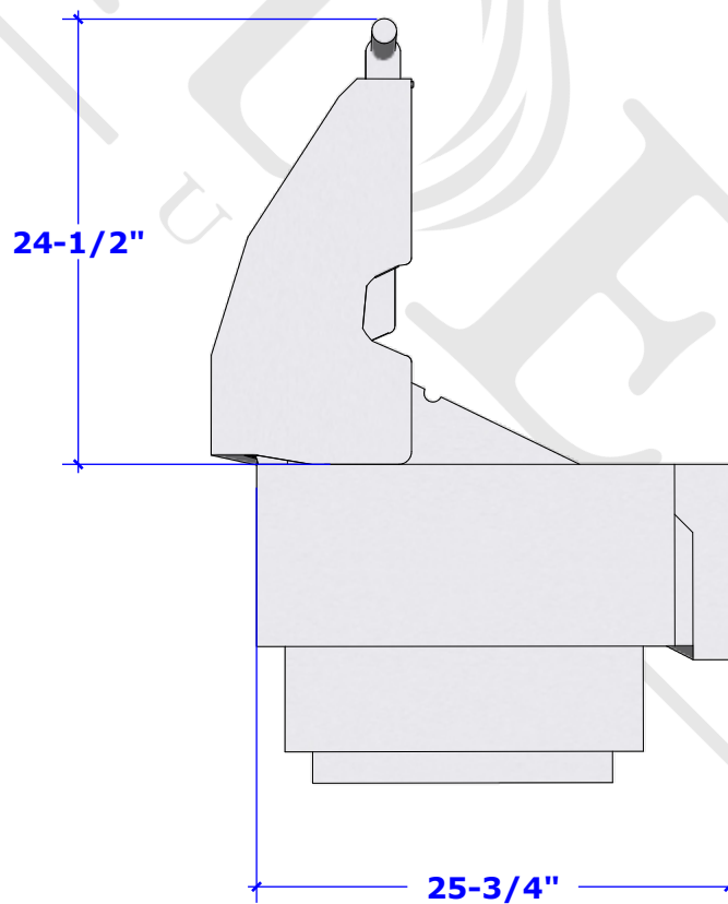
Cut Out Dimension Right Side
