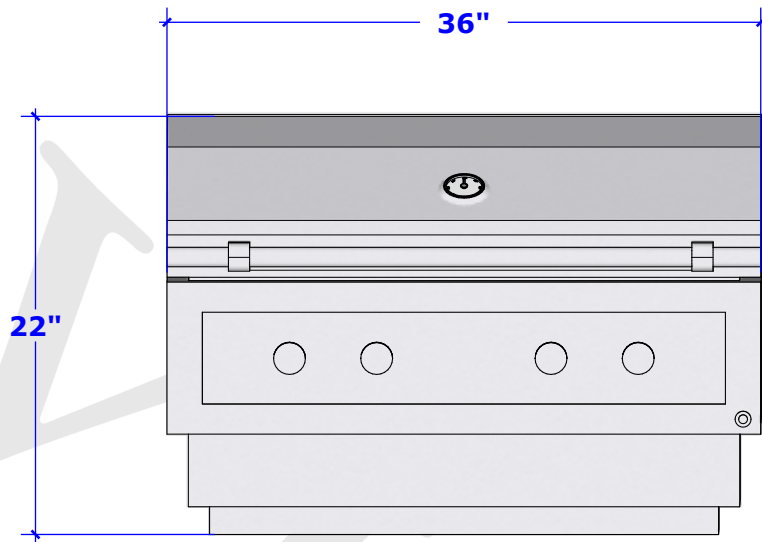
Overall Dimension
